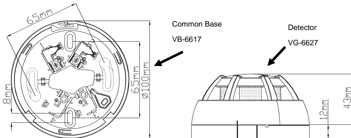
Fig.1 Dimensions
