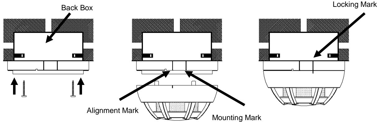
Fig.2 Mounting
